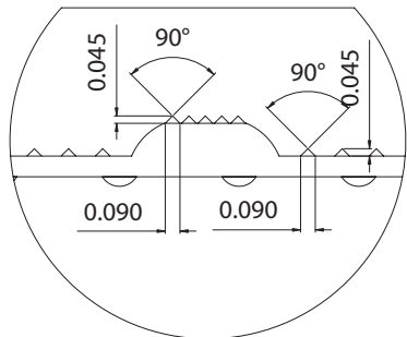
DETAIL "C"
