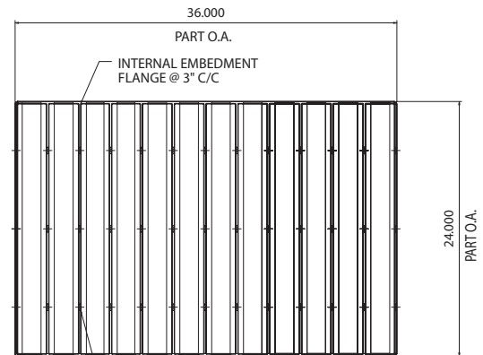
INTERNAL EMBEDMENT FLANGE @ 3" C/C BOTTOM OF PANEL 0.625" DIA. HOLE EMBEDMENT FLANGES
