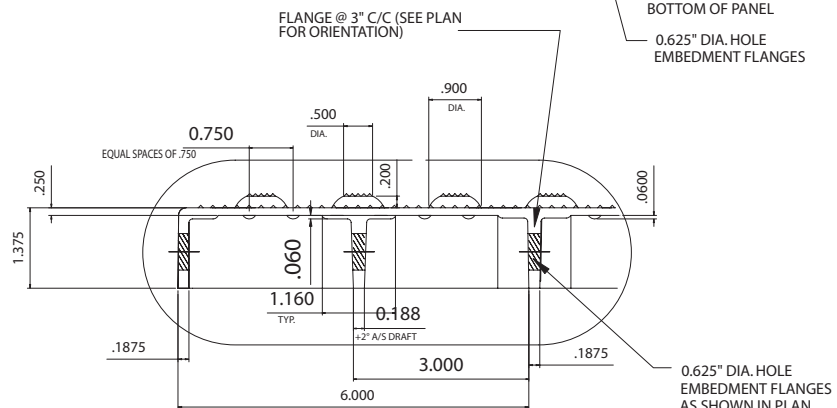
DETAIL "B"
