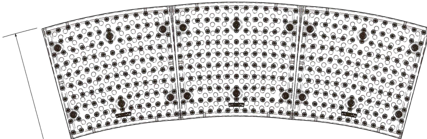
TOP VIEW OF REPLACEABLE PANEL LAYOUT IN A 15' RADII
