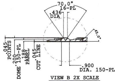
VIEW B 2X SCALE
