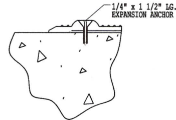
TILE INSTALLATION VIEW-B 4x SCALE
