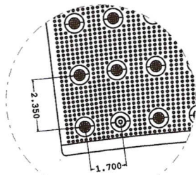
VIEW A 2X SCALE
