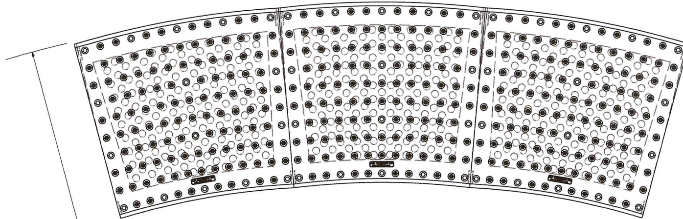
TOP VIEW OF PANELS LAYOUT IN A 15' RADII
